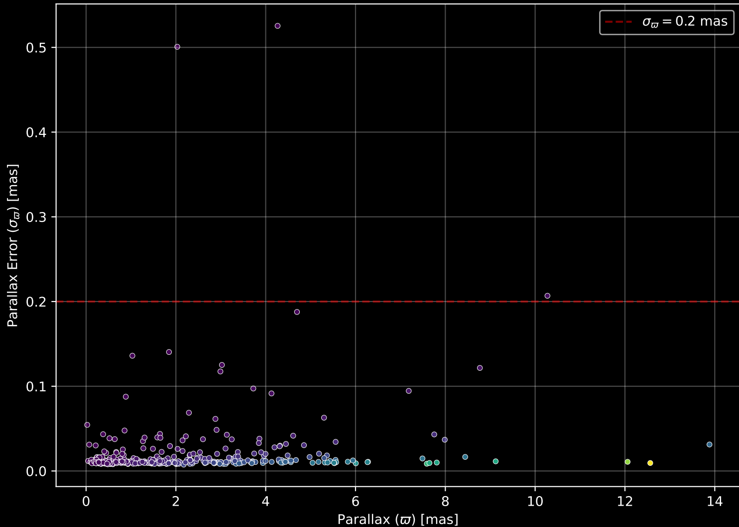
APOGEE DR17 Field: [K13_071+16] Parallax Quality (n= 423)
