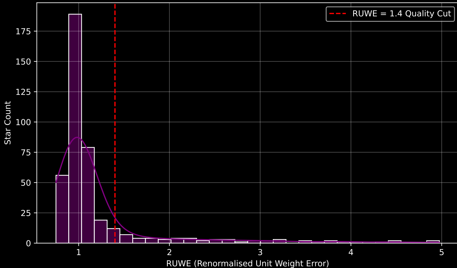
GAPOGEE DR17 Field [K13_071+16] RUWE Distribution (n= 409)
