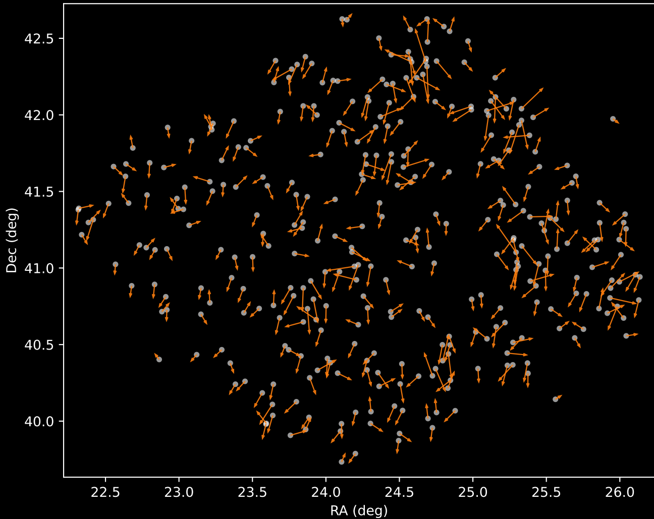
APOGEE DR17 Cluster 2 Proper Motion Vectors (n=333)
