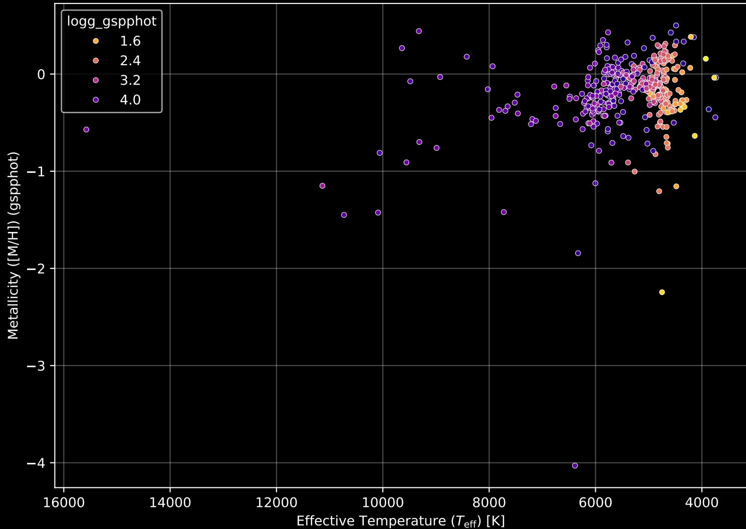
APOGEE DR17 Field: [K13_071+16] Stellar Population Parameters (n= 423)
