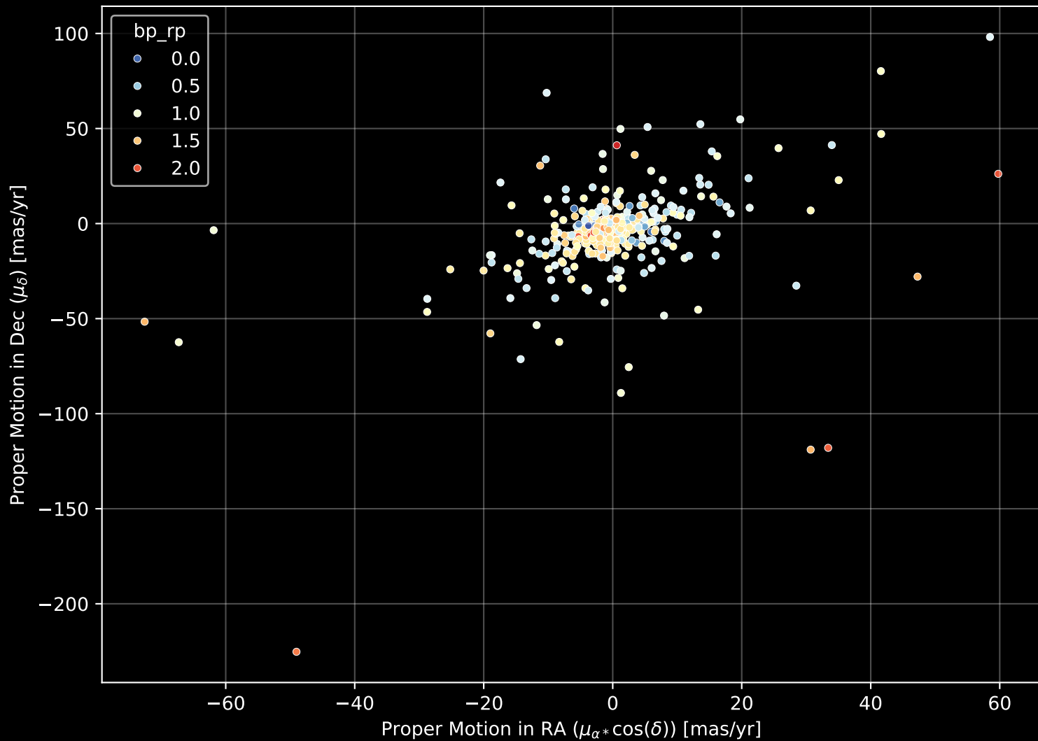
APOGEE DR17 Field: [K13_071+16] Proper Motion Diagram (n= 423)
