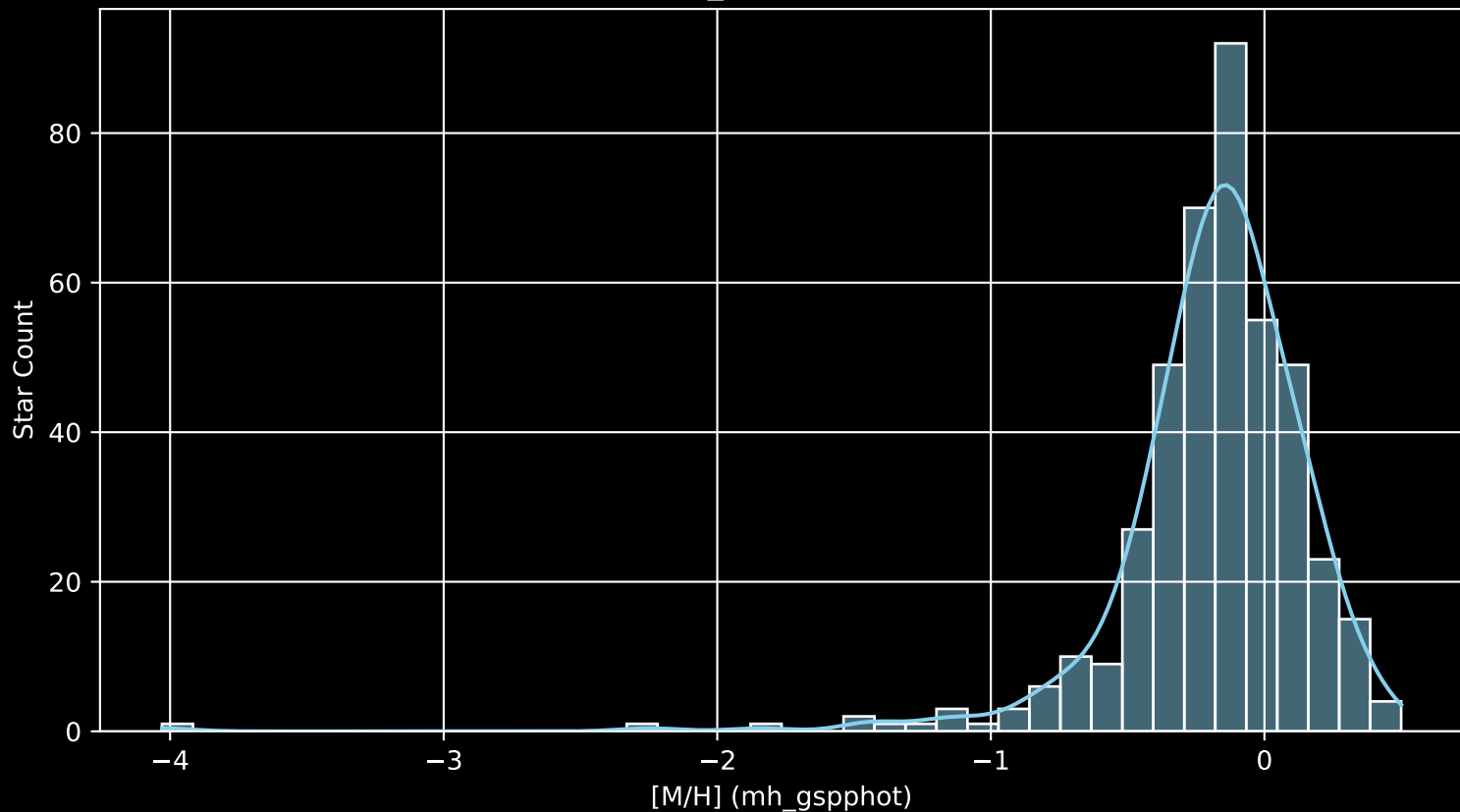
APOGEE DR17 Field: [K13_071+16 [M/H] (mh_gspphot) (n= 423)
